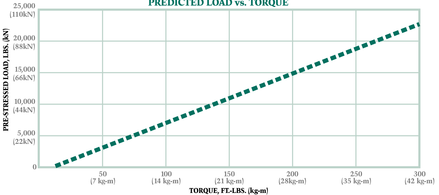
PREDICTED LOAD vs. TORQUE
