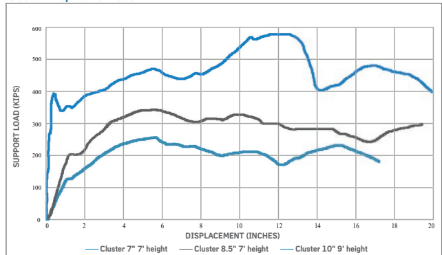
Cluster Prop Performance
